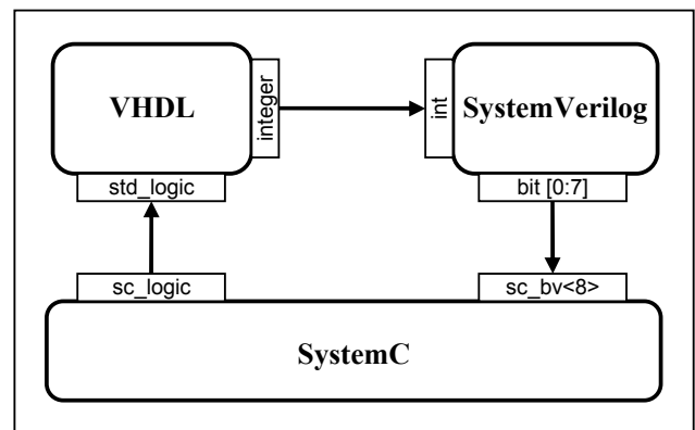
Figure 1: Using types across the boundary
