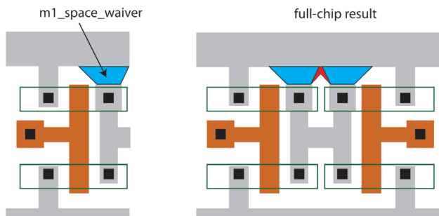
Waivers that become modified in context are identified through pattern matching criteria defined by the foundry.
